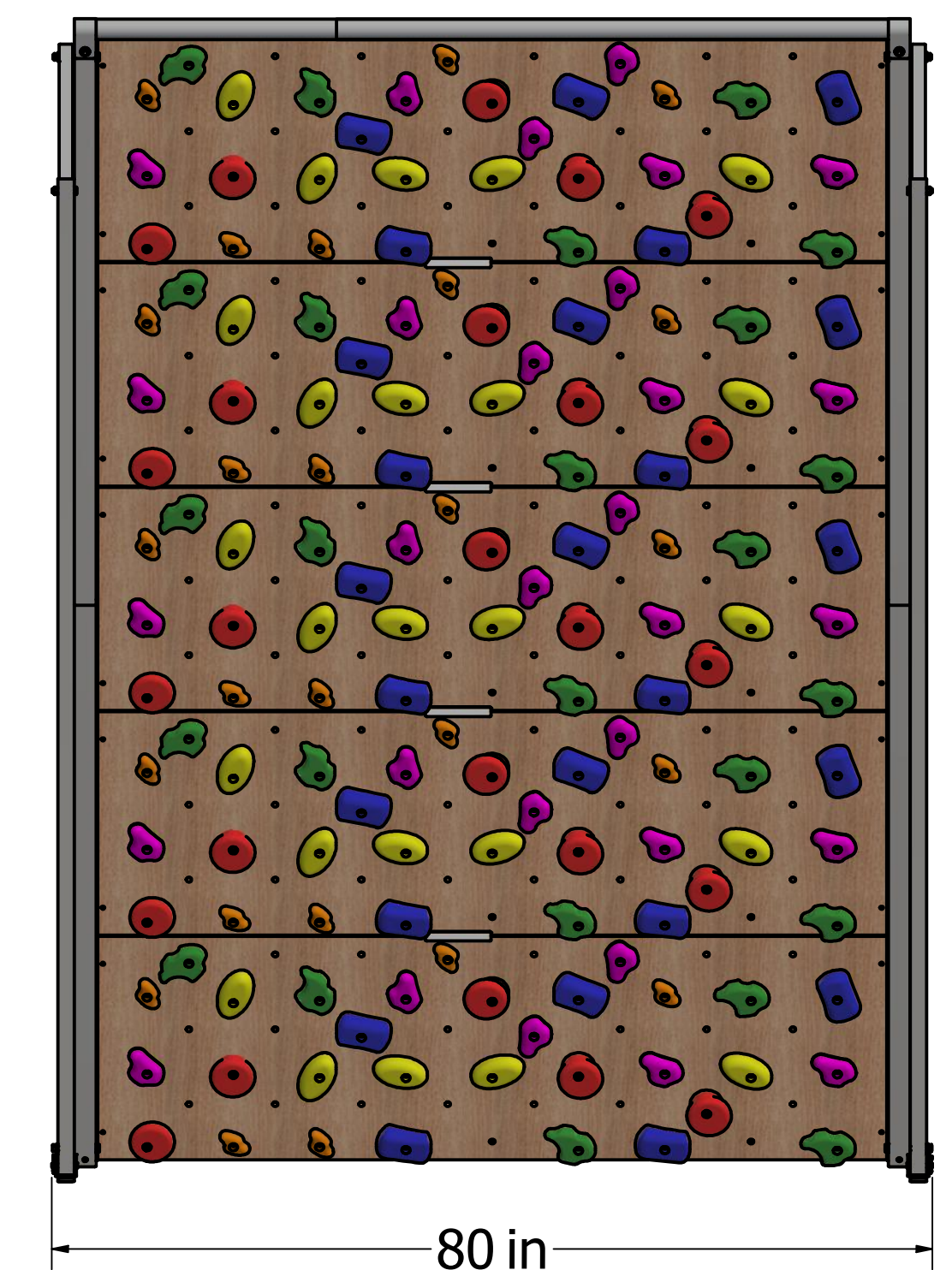
Front View
